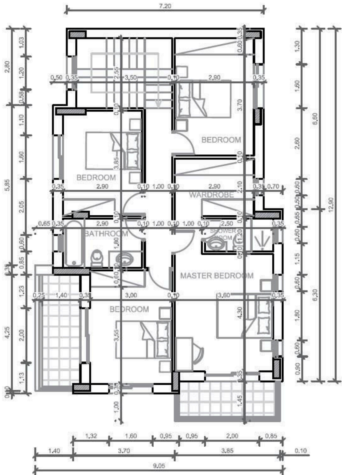
FIRST FLOOR HOUSE B
