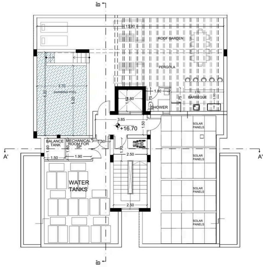
ROOF PLAN
