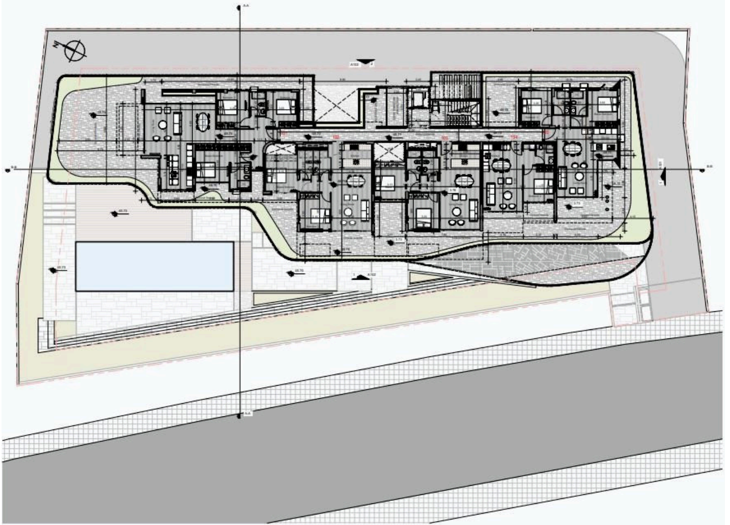
A002-FIRST FLOOR 1:100
