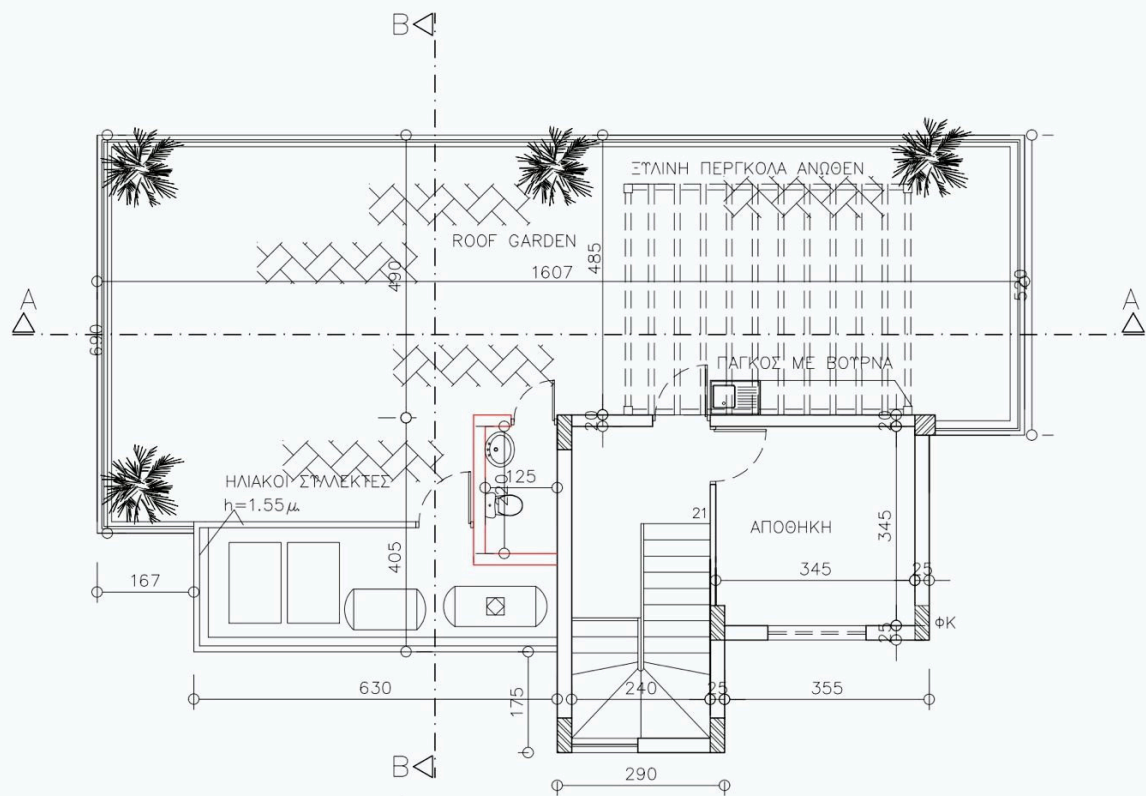
ROOF GARDEN PLAN
