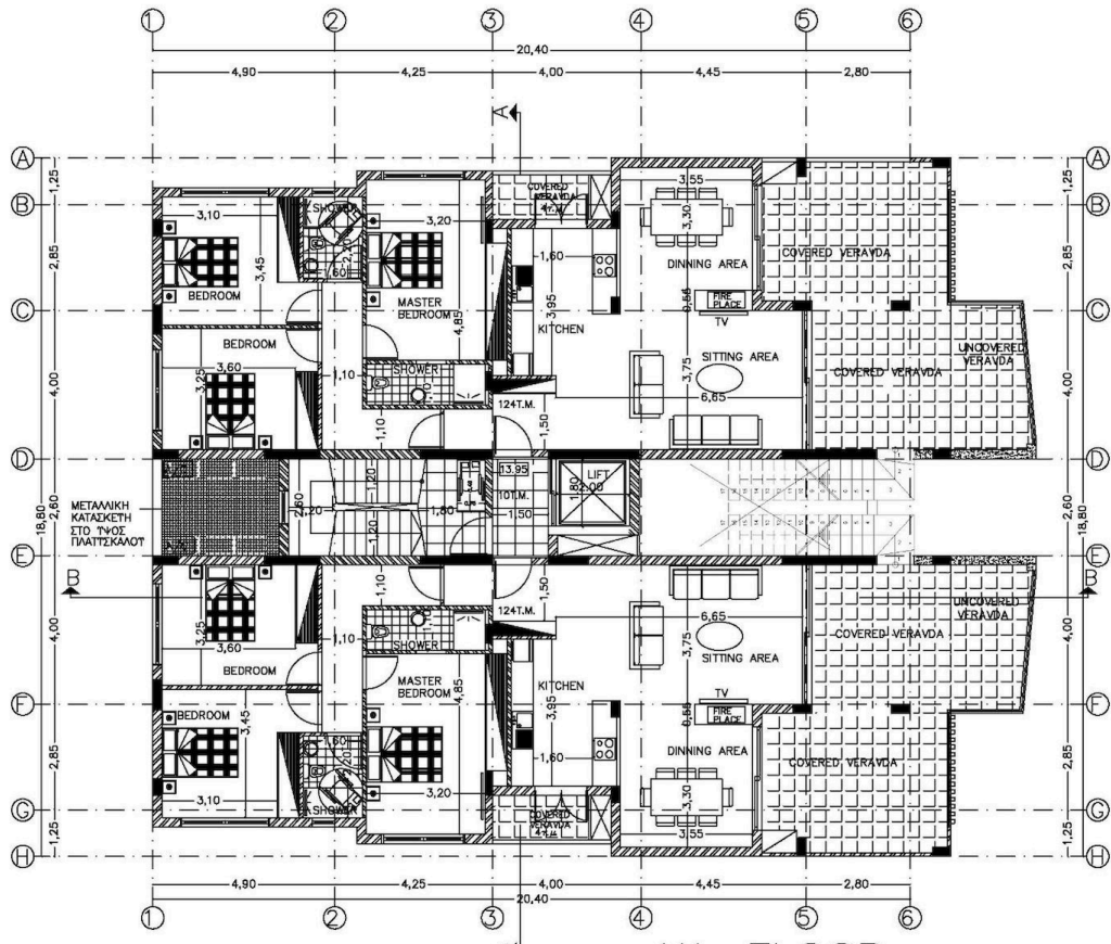
4th FLOOR
