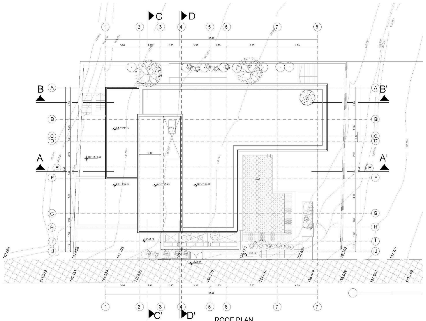
ROOF PLAN 1:100
