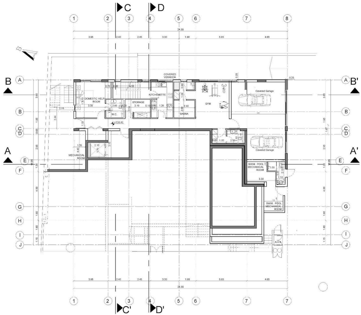
BASEMENT 1:100
