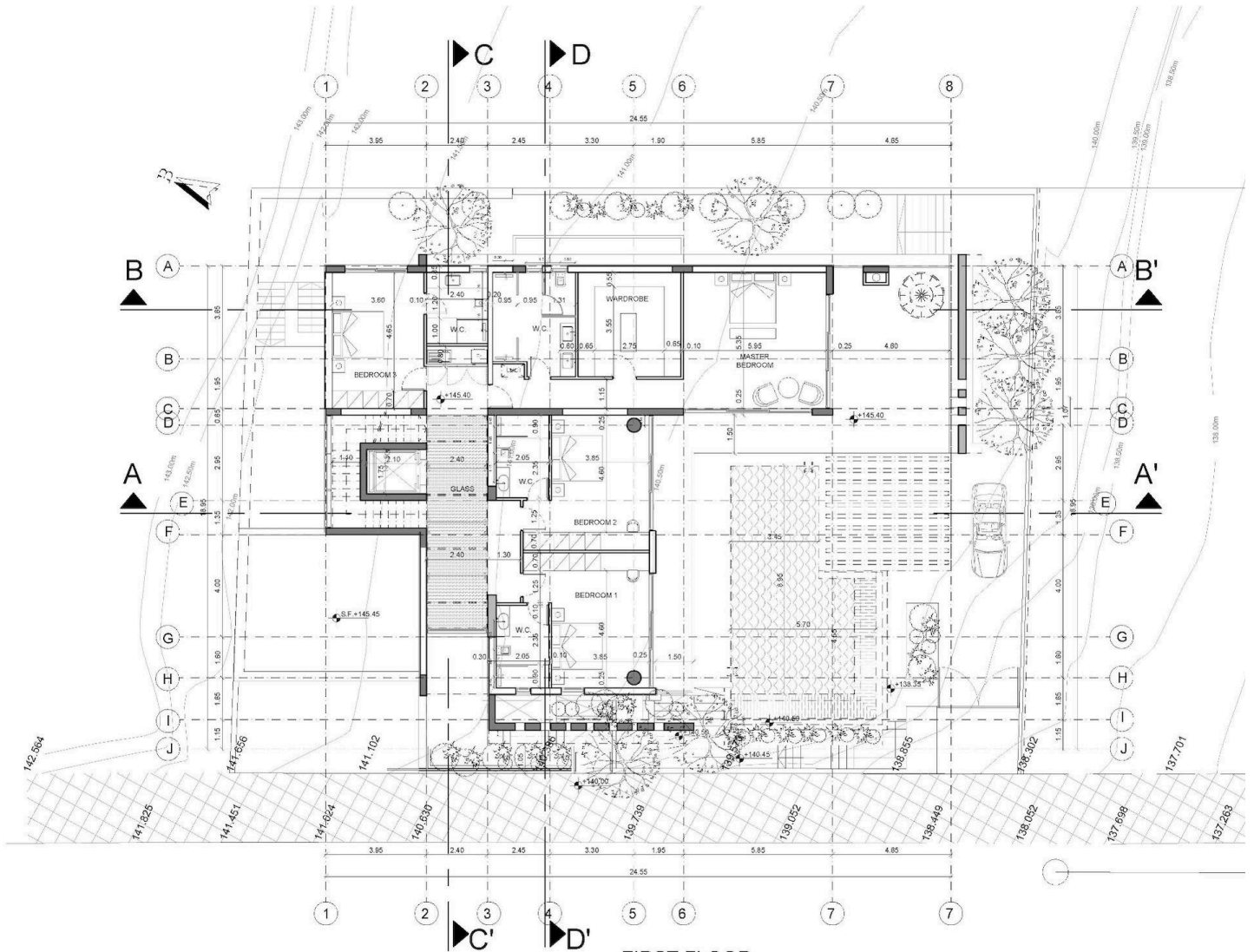
FIRST FLOOR 1:100
