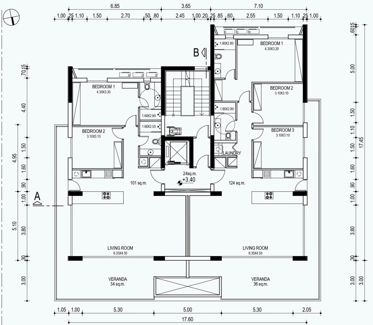
5th FLOOR PLAN
