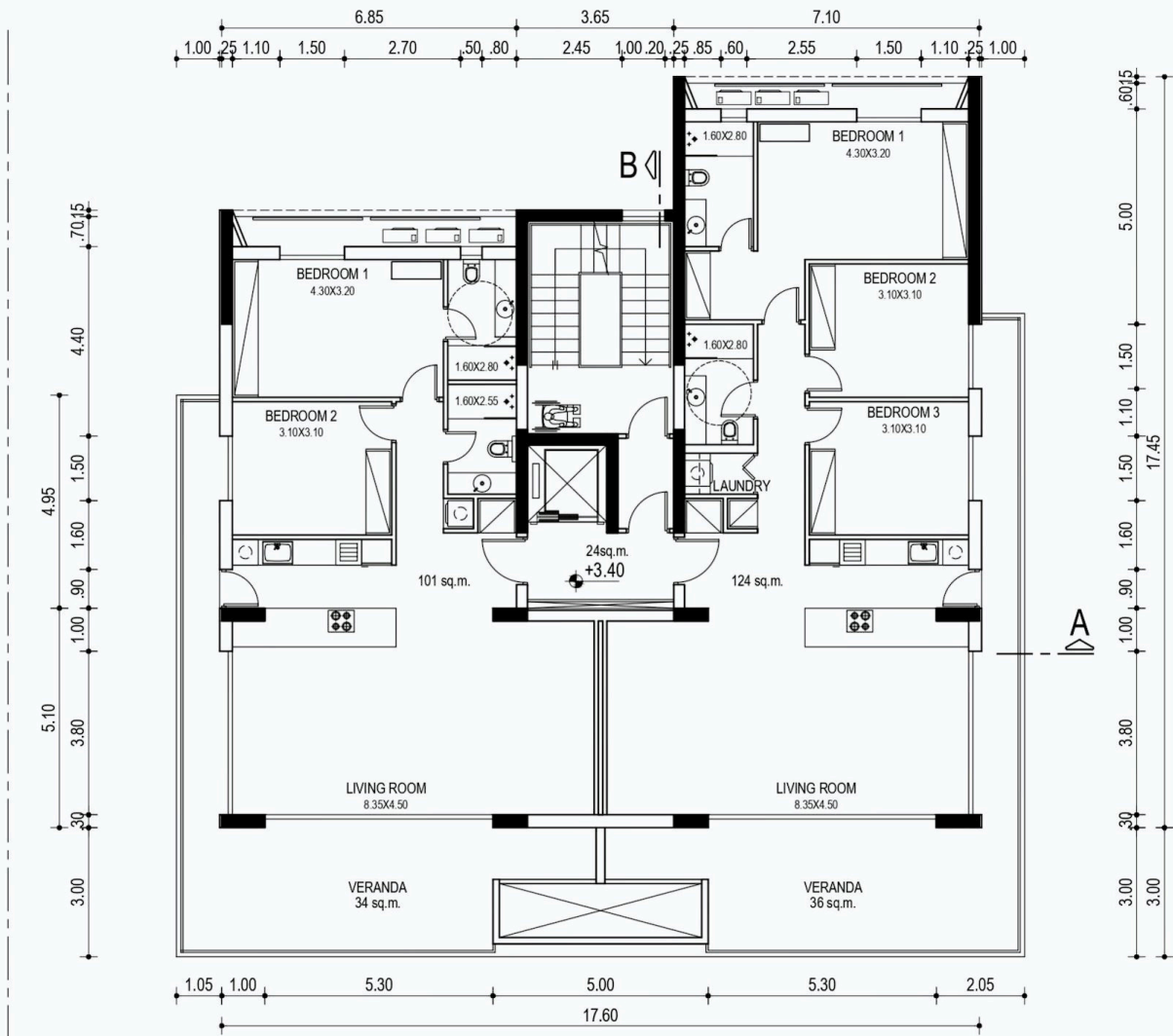
6th FLOOR PLAN
