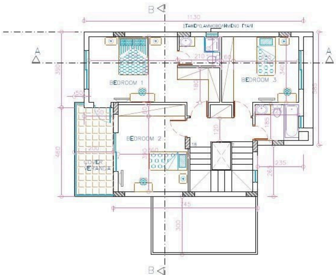
1ST FLOOR PLAN HOUSE 2
