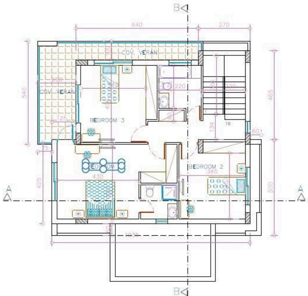
1ST FLOOR PLAN HOUSE 1
