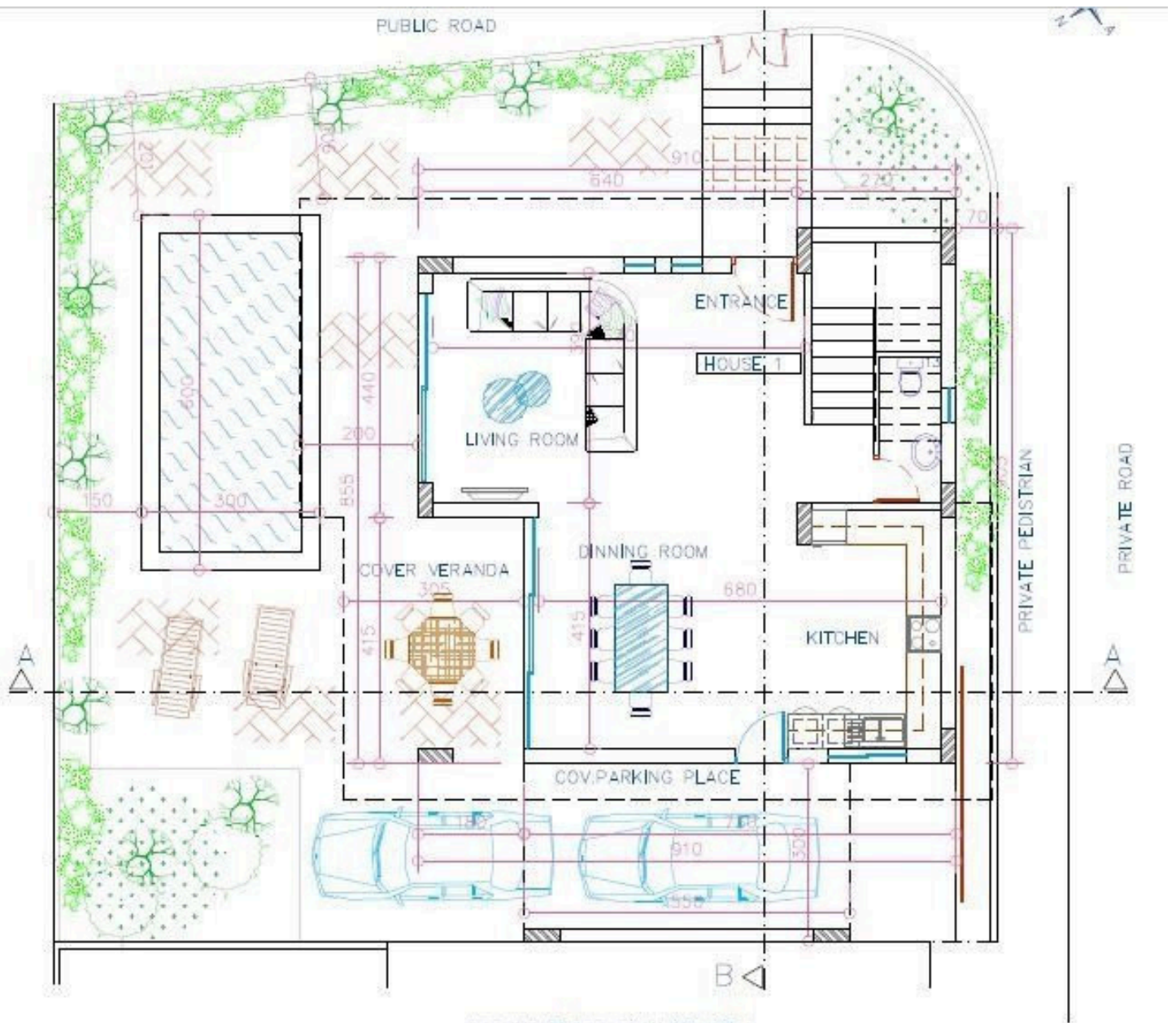
GROUND FLOOR PLAN HOUSE 1
